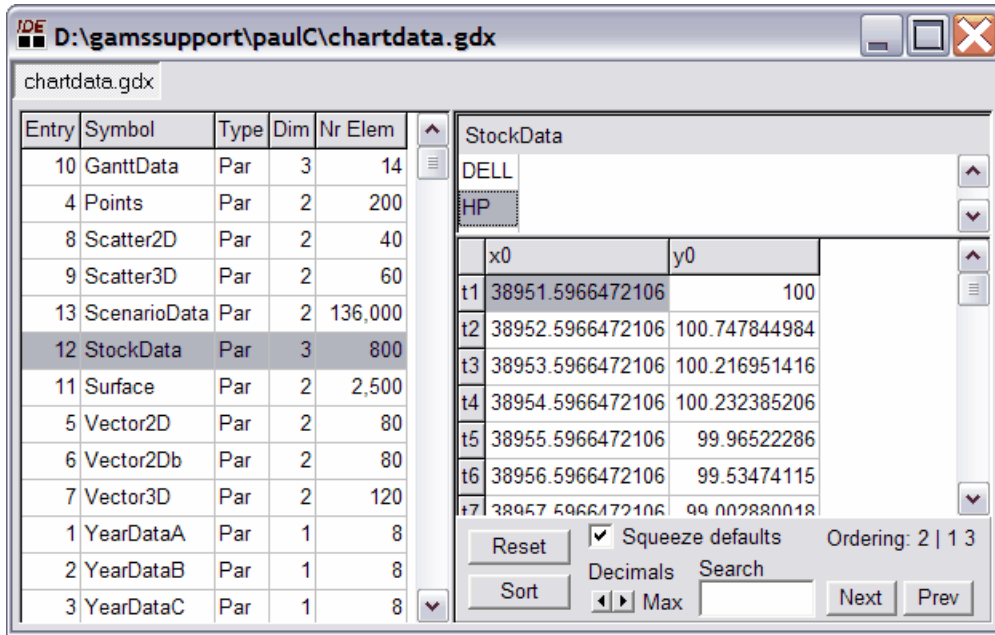
StockData with filter for HP
